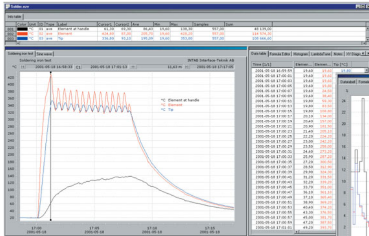
The soldering iron test shows tip temperature. The oscillations around 360°C show how the thermostat works.
